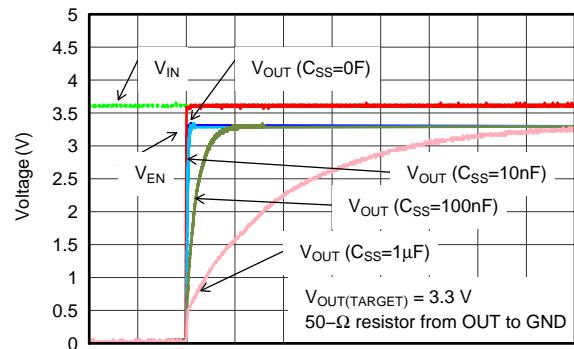
Time (50 ms/div)
