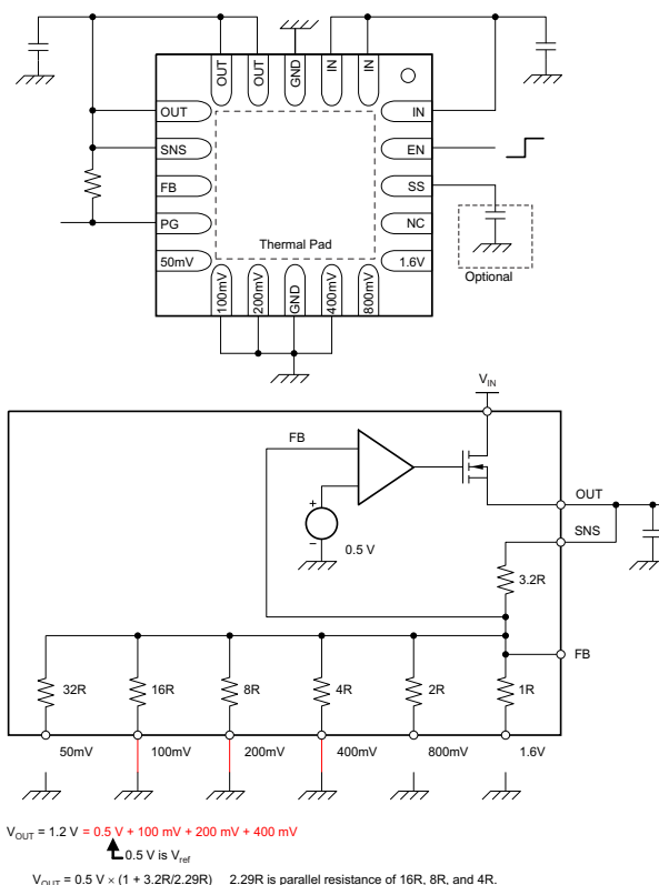
Figure 35. 1.2-V Configuration
