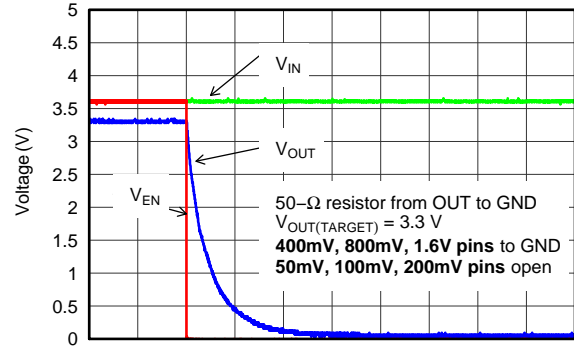
Time (1 ms/div)
