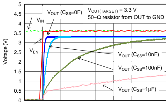
Time (5 ms/div)
